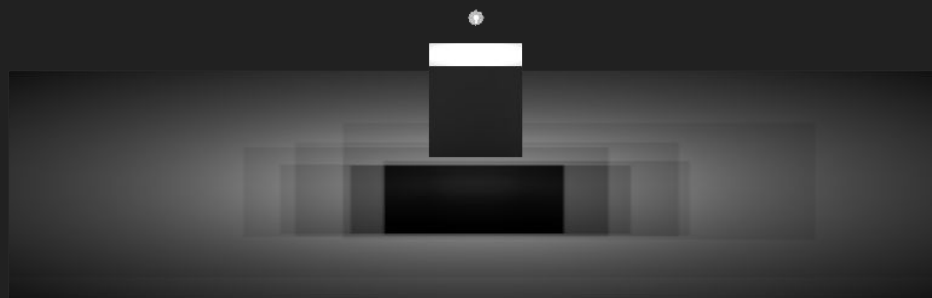
8 Samples (Default)
