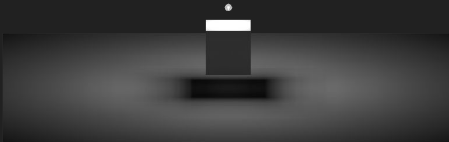
512 Samples
